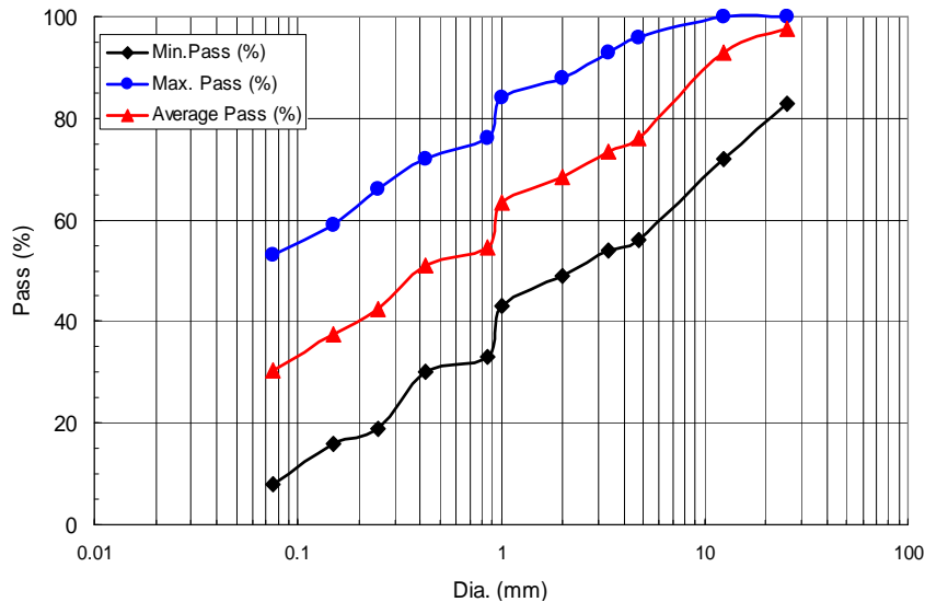
Figure 6: Maximum, Minimum and Average Grain Size Distribution Curves of Soil around Arar's City
